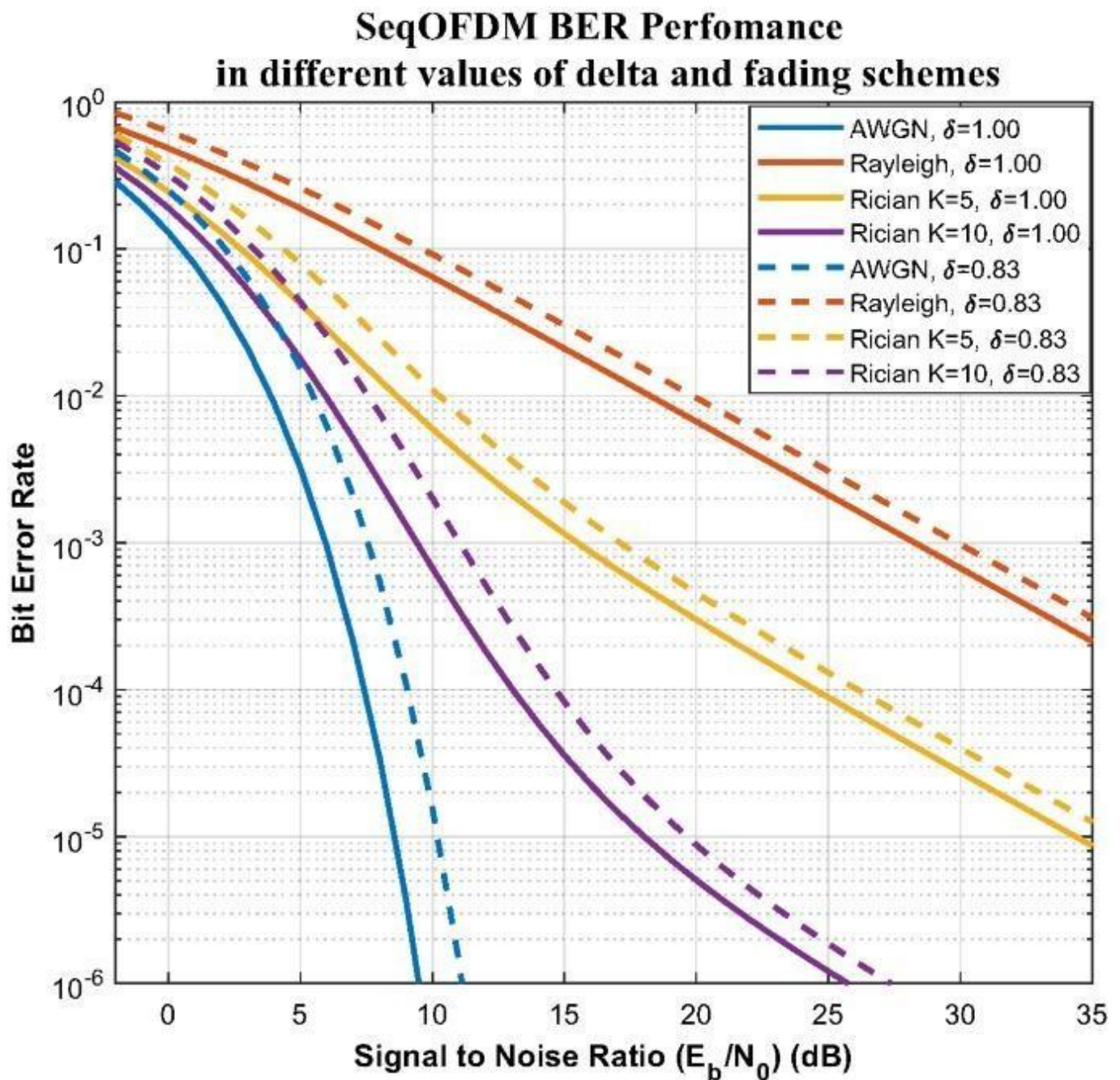
Graph 1: BER vs SNR
